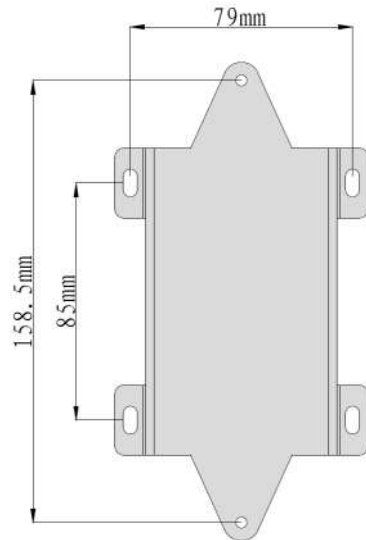
Figure 4: Mounting Bracket
