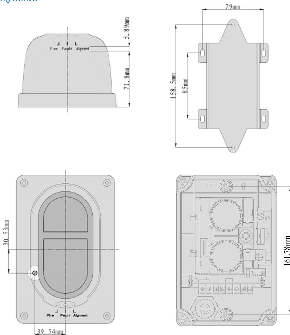
Figure 2: Detector Diagram
